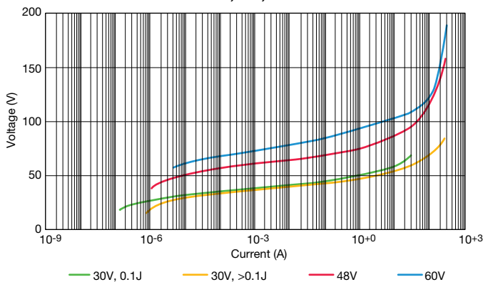
VI Curves - 30V, 48V, and 60V Products
