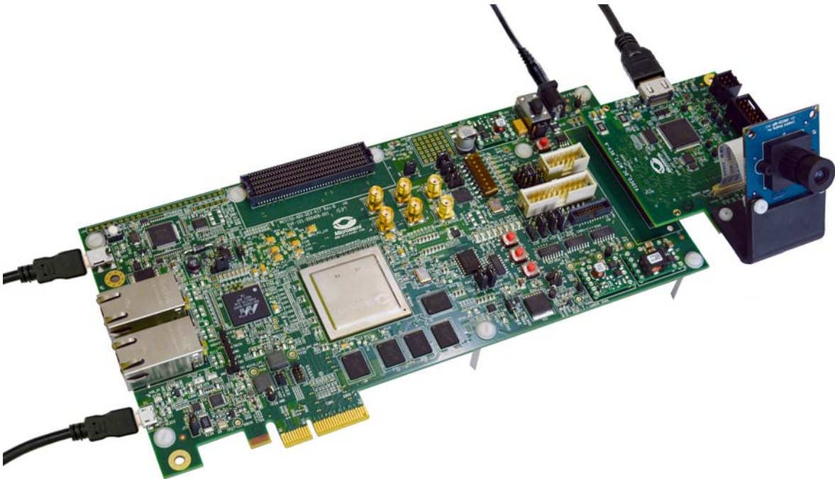
Figure 5 • Hardware Setup
