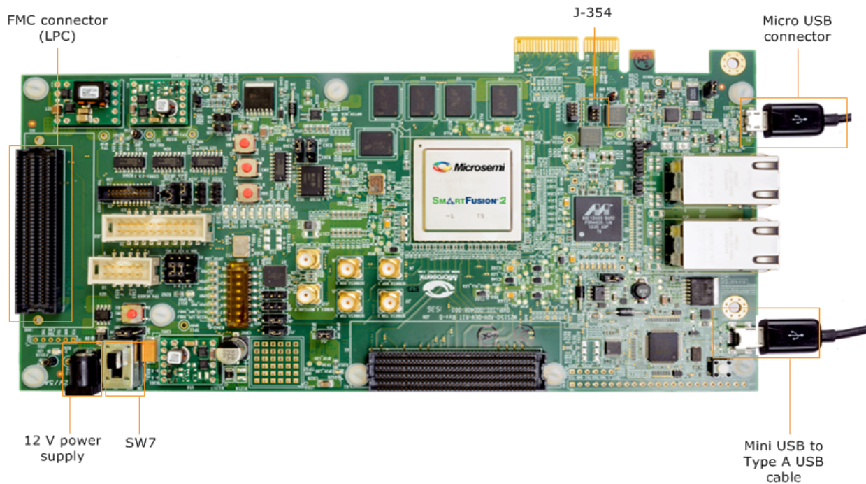
Figure 8 • SmartFusion2 Advanced Development Kit Setup
