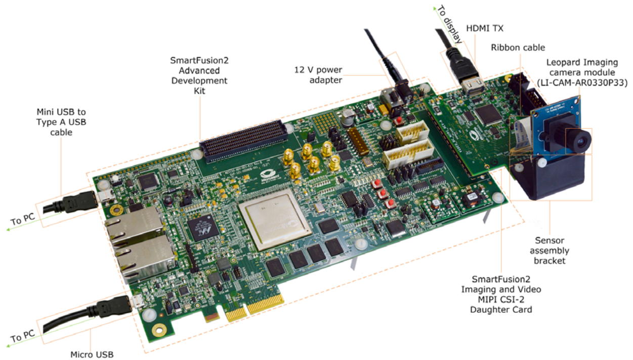
Figure 2 • Full Setup
