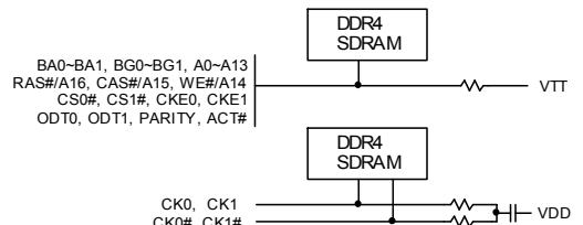
Command, address, control, and clock line terminations
