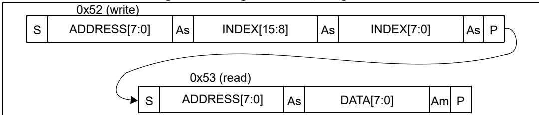
Figure 25. Single location, single read
