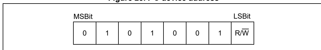
Figure 23. I 2 C device address
