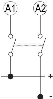
Fig. 21 Power supply
