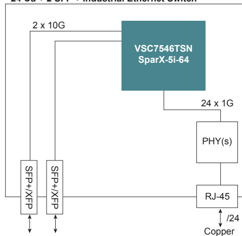
24 Cu + 2 SFP + Industrial Ethernet Switch
