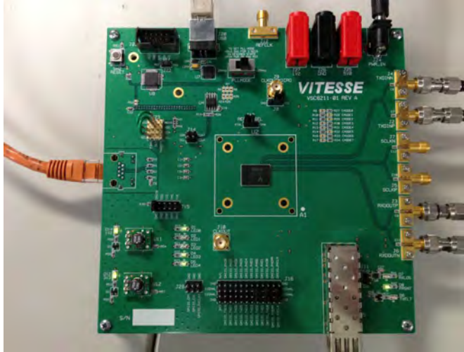
Figure 1 • VSC8211EV
