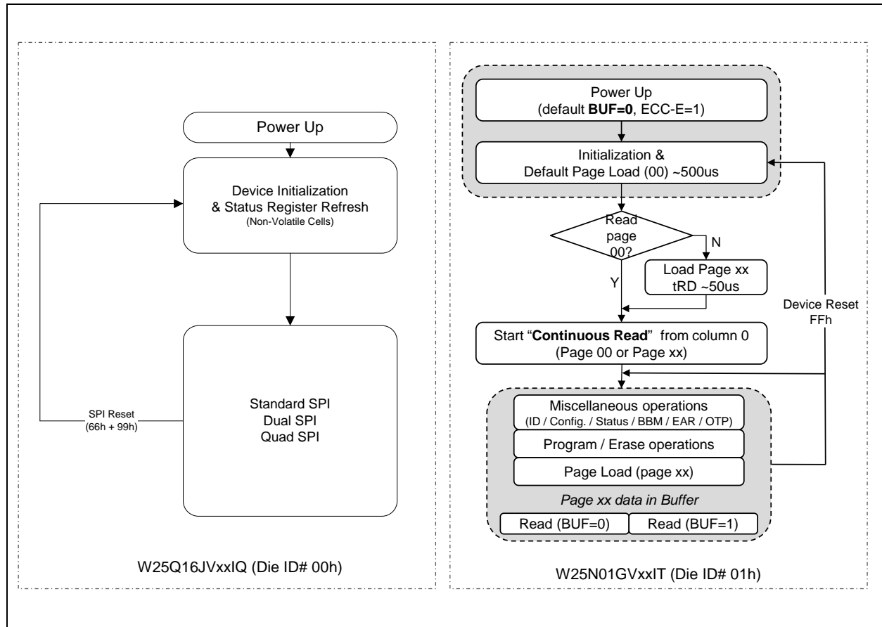
Figure 5. W25M161AV Software Reset Operation Flow
