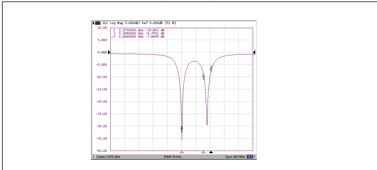
(Return Loss)
