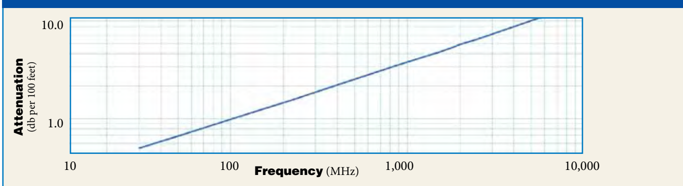
Attenuation vs. Frequency (typical)
