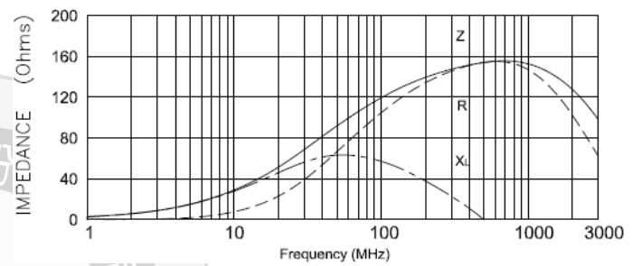
WLBD0603HCU121TL
