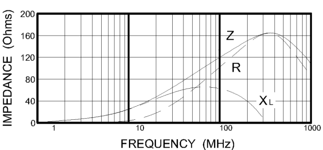
WLBD2012K2U121TP
