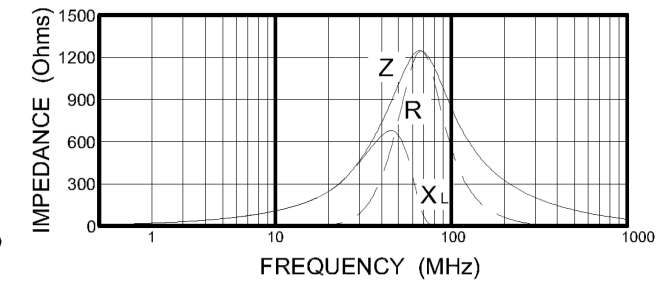
WLBD3225HCU102PH
