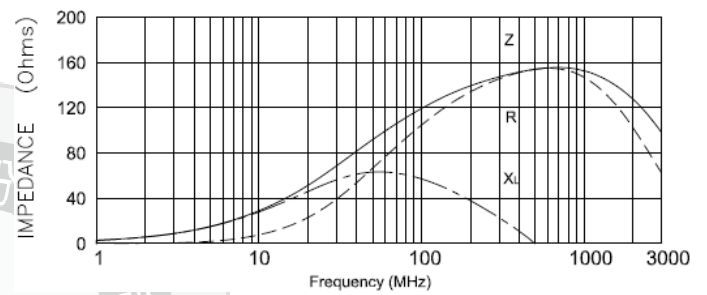
WLBD0603HCU121TL
