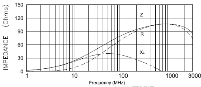
WLBD0603HCU800TL
