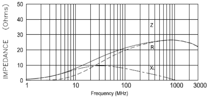
WLBD0603HCU220TL
