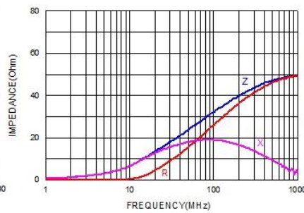
WLBD3216K1U700PB
