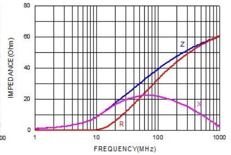
WLBD3216K1U900PB
