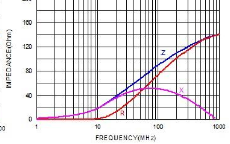
WLBD3216K1U900PB
