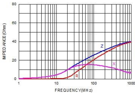
WLBD3216K1U500PB
