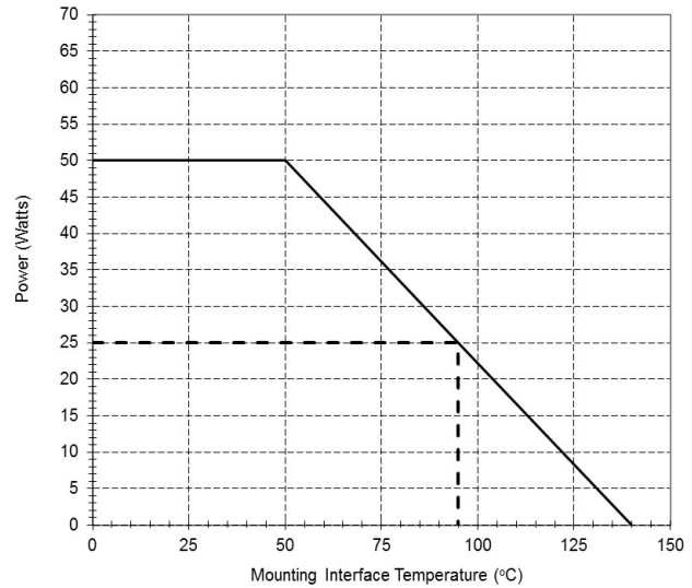
X3C25F1-03S Power Derating Curve
