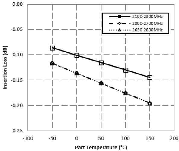
X3C25F1-03S Typical Insertion Loss Derating Curve
