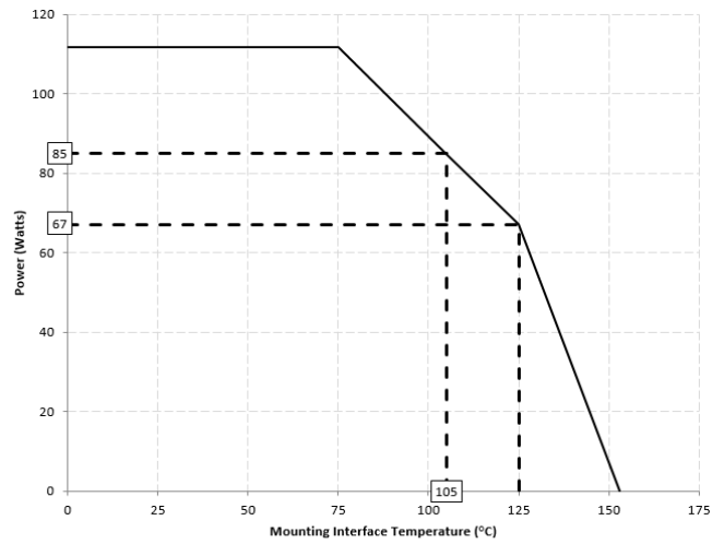
X3C35P1-03S Power Derating Curve
