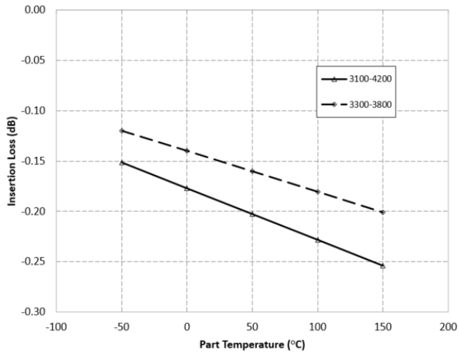
X3C35P1-03S Typical Insertion Loss Derating Curve
