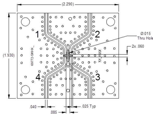
2dB, 3dB, 4dB and 5dB Test Board
