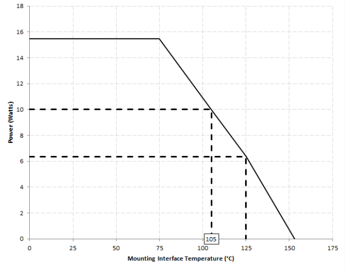
X4C20K1-03S Power Derating Curve
