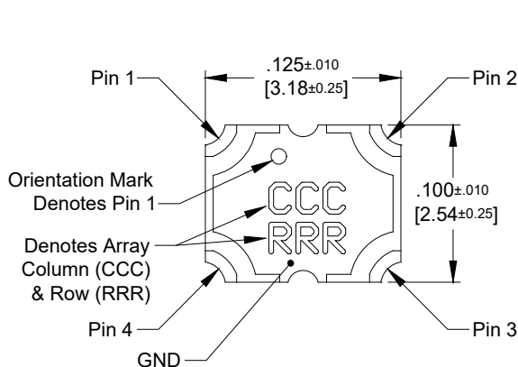
Dimensions are in Inches [Millimeters] X4C20K1-03S Mechanical Outline
