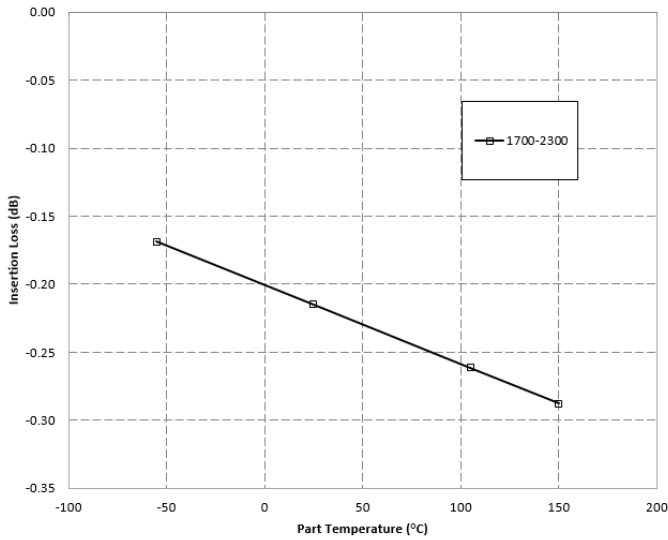
X4C20K1-03S Typical Insertion Loss Derating Curve
