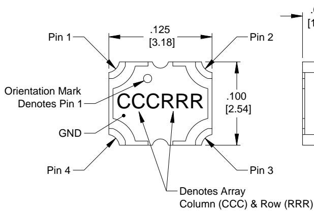
Dimensions are in Inches [Millimeters] Mechanical Outline X4C25K1-03S
