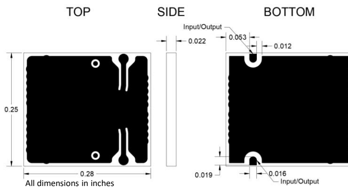
6 pole BPF Footprint
