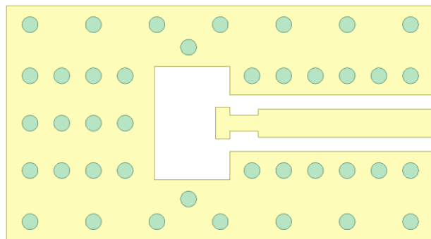
Test Board is 5mil RO3003
