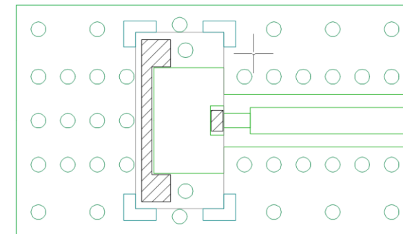
Hashed area show mounting footprint
