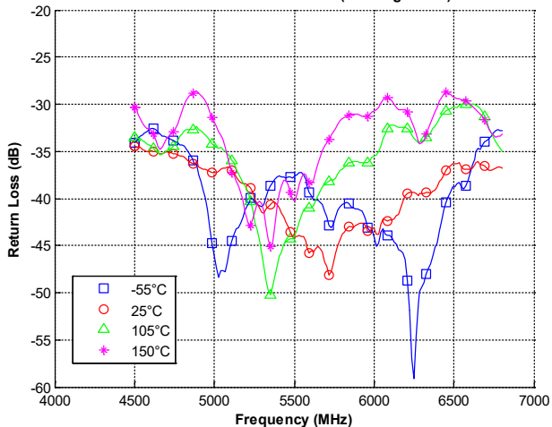
Return Loss for X4C55K1-03S (Feeding Port 1)
