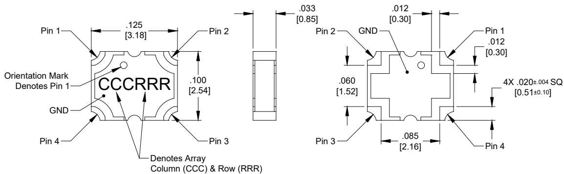
Dimensions are in Inches [Millimeters] Mechanical Outline X4C55K1-03S
