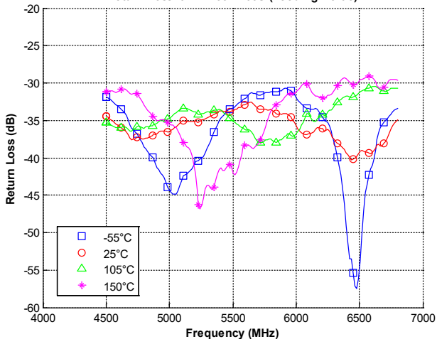
Return Loss for X4C55K1-03S (Feeding Port 3)
