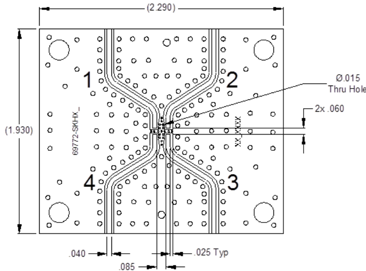
2dB, 3dB, 4dB and 5dB Test Board
