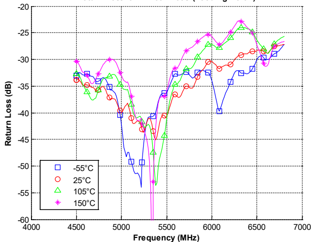
Return Loss for X4C55K1-03S (Feeding Port 4)
