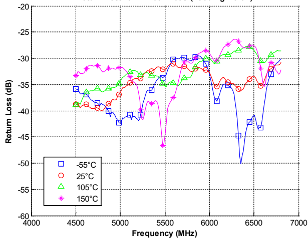
Return Loss for X4C55K1-03S (Feeding Port 2)
