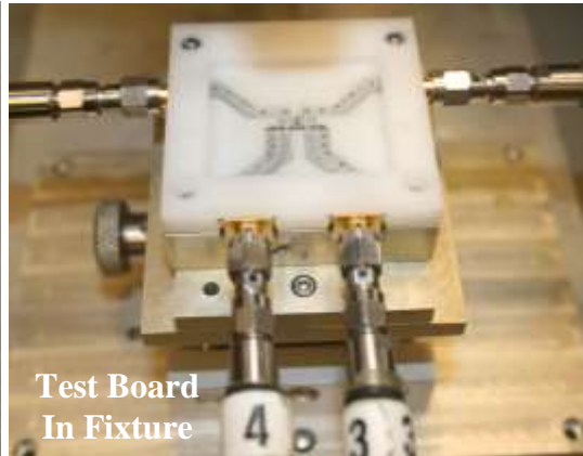
Test Station
