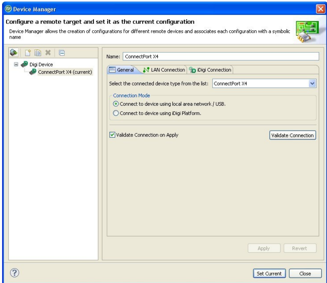
Figure 22: Device Manager
