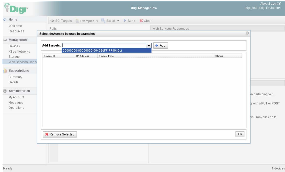
Figure 44: Add Targets
