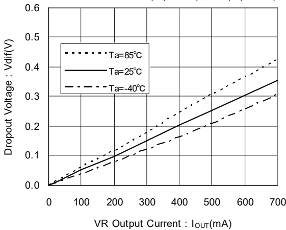
XC6210x302xx
