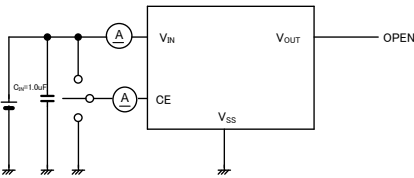
Circuit ②
