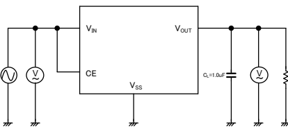
Circuit ③
