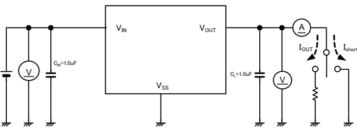
Circuit ②
