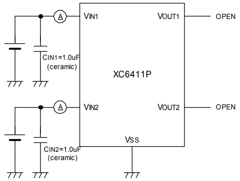
Circuit ②
