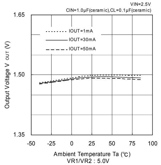
VR1/VR2: 5.0V
