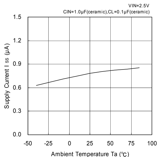
VR1/VR2: 1.5V
