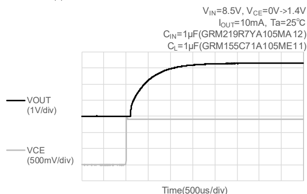
(14-2) V_{OUT(\tau)}=3.3V
