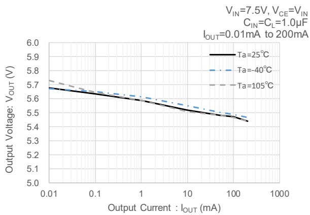
(8-3) V_{OUT(T)}=5.5V
