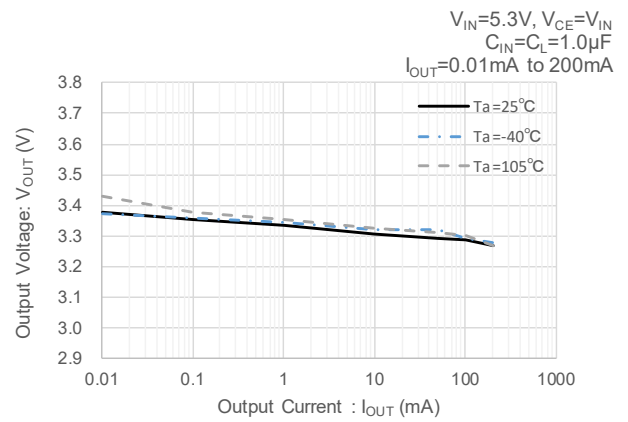
(8-2) V_{OUT(T)}=3.3V
