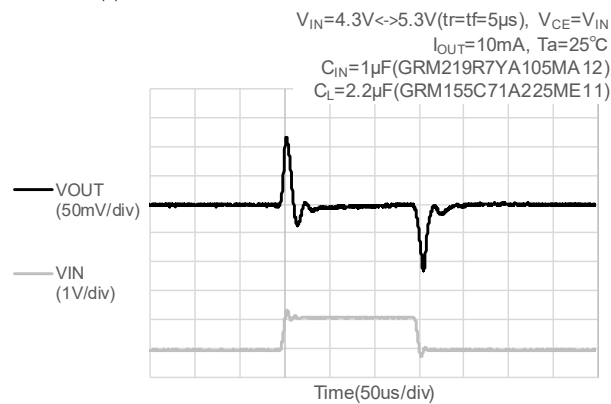
(17-2) V_{OUT(T)}=3.3V
