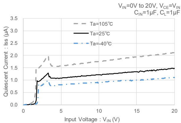
(1-2) V_{OUT(T)}=3.3V
