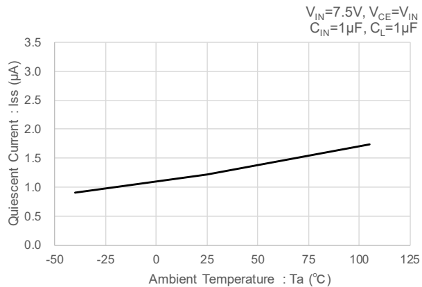
(2-3) V_{OUT(T)}=5.5V
