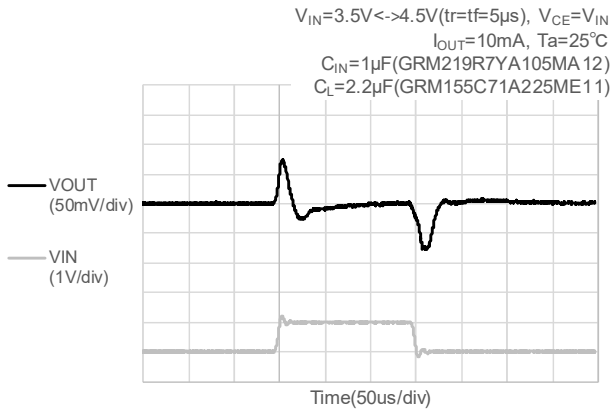
(17-1) V_{OUT(T)}=2.5V
