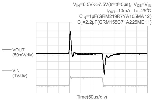
(17-3) V_{OUT(T)}=5.5V
