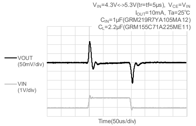
(17-2) V_{OUT(T)}=3.3V
