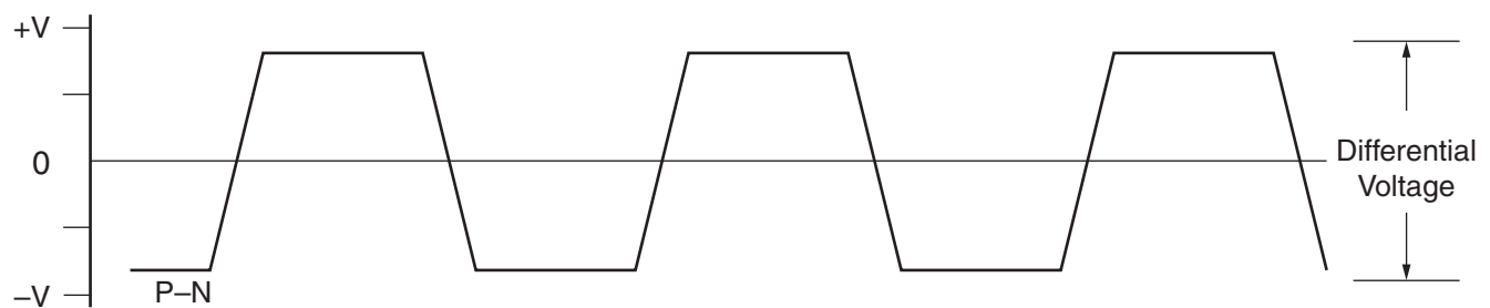
Figure 12: Differential Peak-to-Peak Voltage
