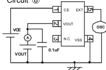
Circuit ⑧
