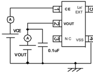
Circuit ⑥
