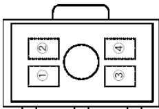
SOT-89 (TOP VIEW)
