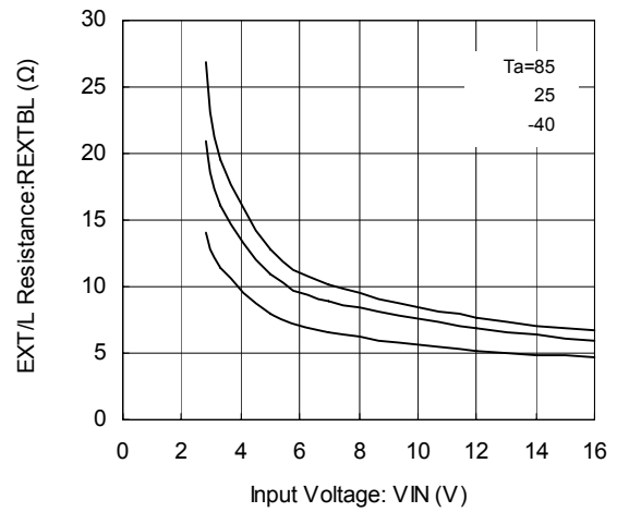
XC9220/21 Series
