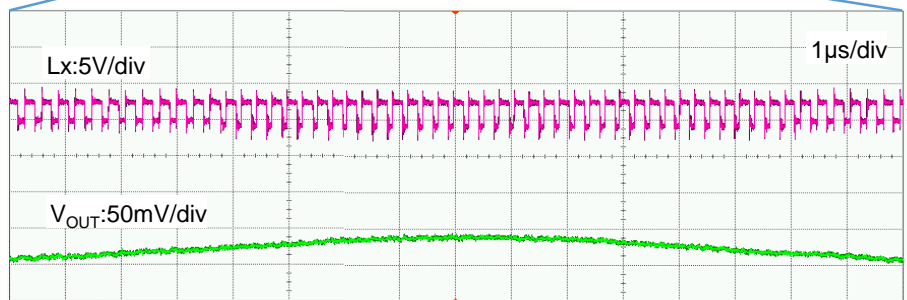
Fig Unstable operation in heavy load
