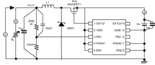
Circuit ⑤
