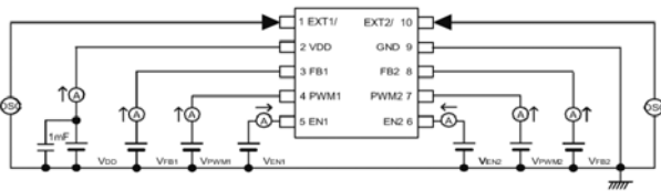
Circuit ③
