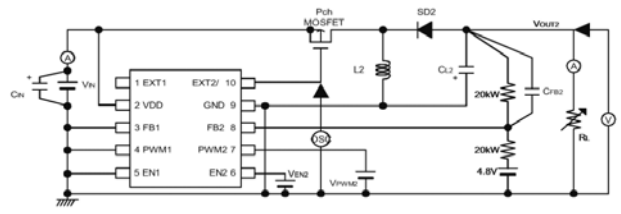
Circuit ⑥
