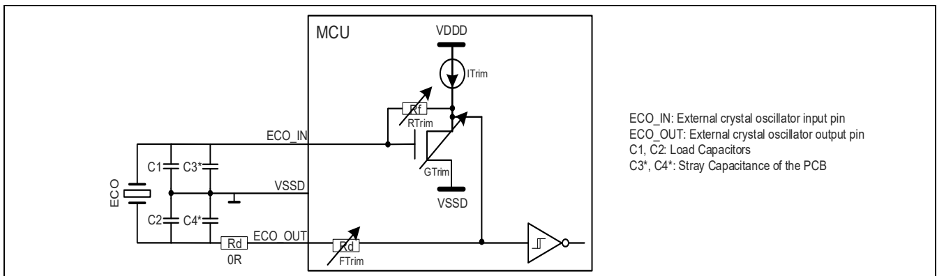
Figure 26-22 ECO connection scheme [70]
