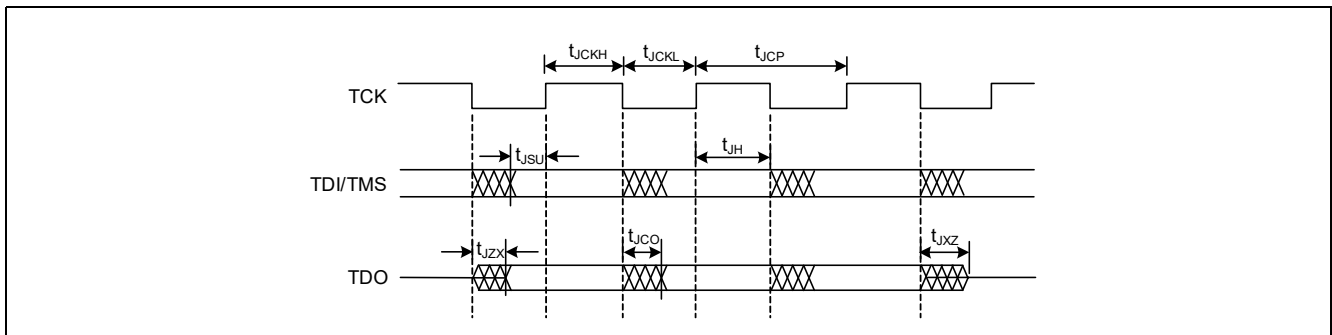
Figure 26-21 JTAG specifications
