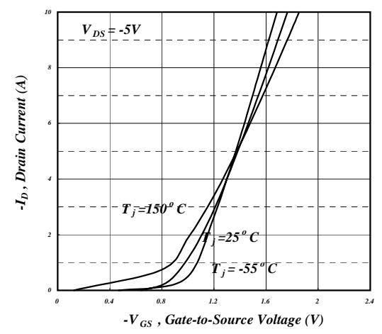
Fig 12. Transfer Characteristics
