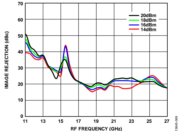
Figure 61. Image Rejection vs. RF Frequency at Various LO Drives, TA = 25°C
