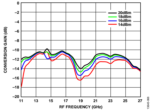
Figure 60. Conversion Gain vs. RF Frequency at Various LO Drives, TA = 25°C
