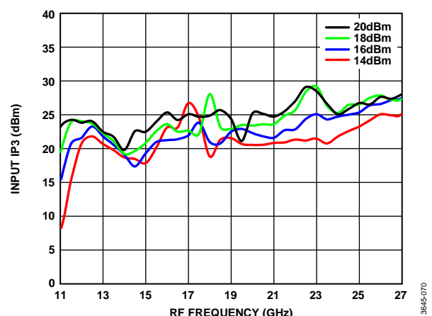
Figure 62. Input IP3 vs. RF Frequency at Various LO Drives, TA = 25°C
