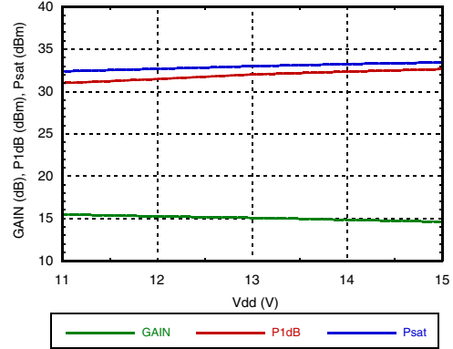
Gain & Power vs. Vdd @ 10 GHz
