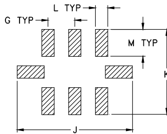
Suggested Layout, Tolerance to be within .002
