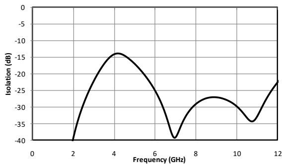
Fig. 4. Isolation.
