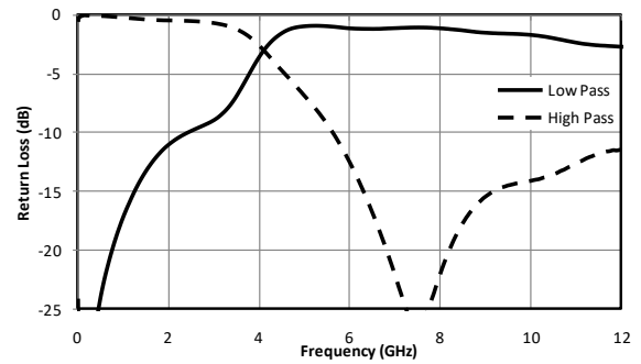
Fig. 3. Return loss.
