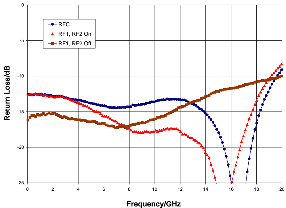
Return Loss
