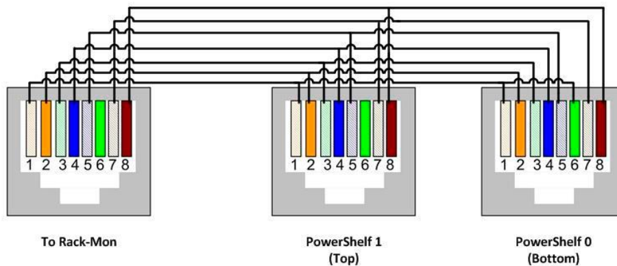
Figure 2. Communication Wiring
