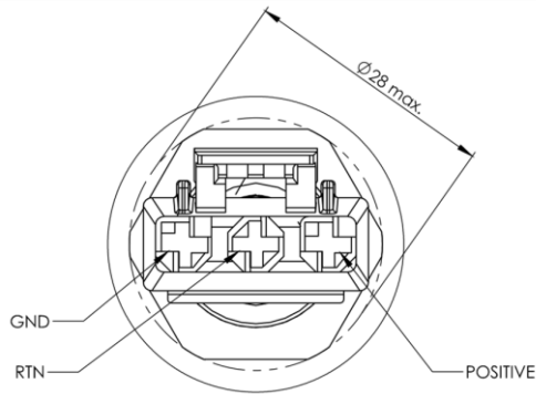
Figure 3. Molex 44441-2003
