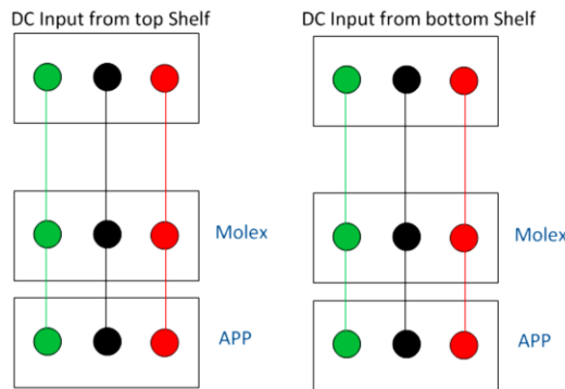
Figure 1: Electrical Schematic
