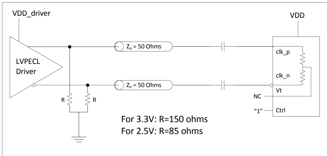
Figure 6 - Clock Input - LVPECL - AC Coupled
