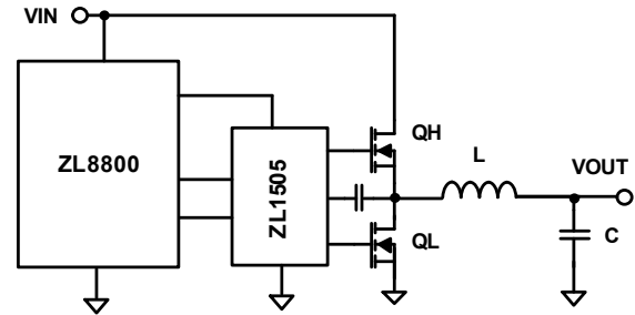
FIGURE 12. SYNCHRONOUS BUCK CONVERTER
