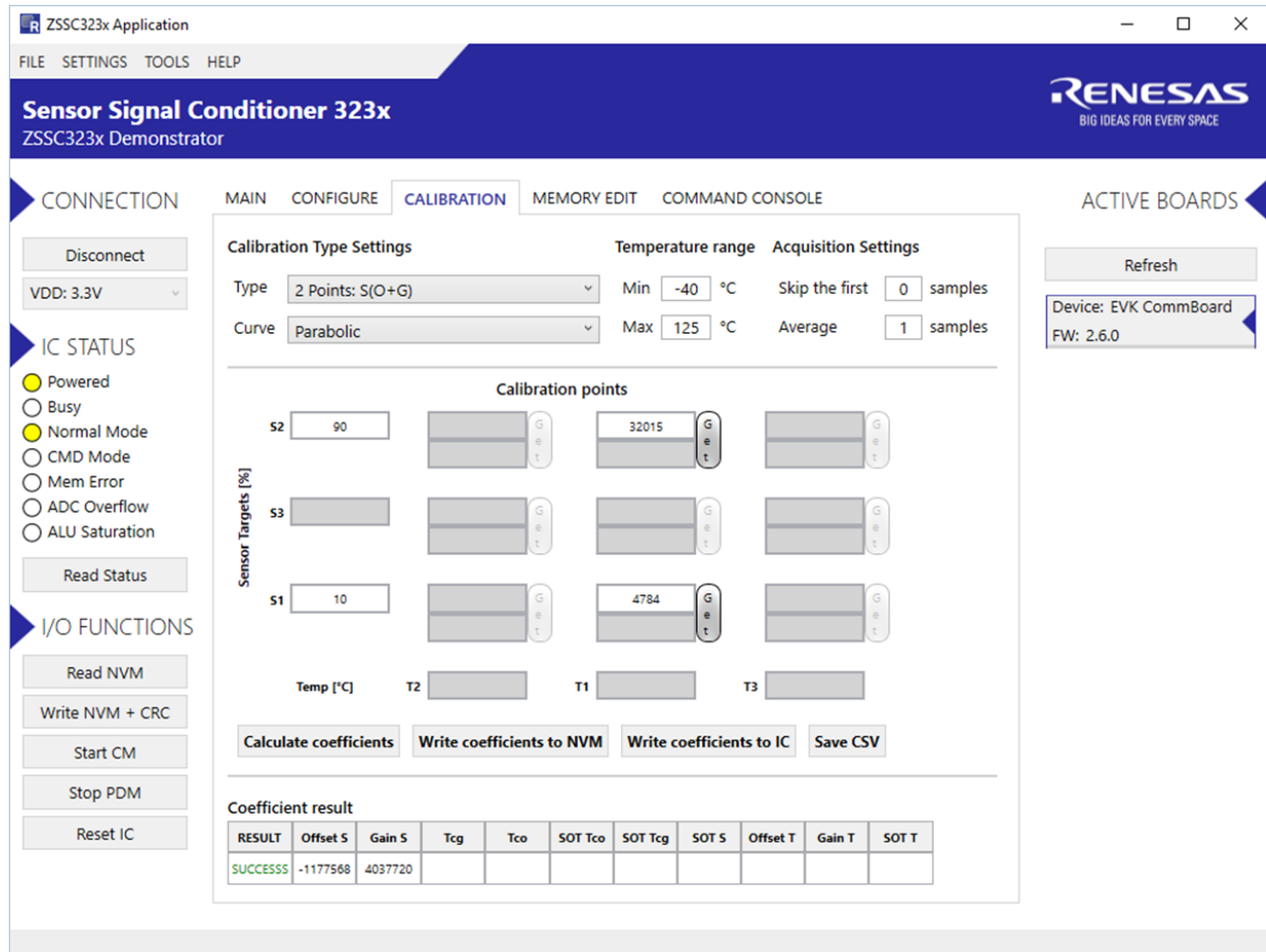
Figure 24. Coefficients Calculation
